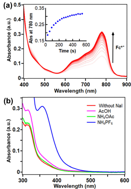
Fig. 3 (a) Evolution of the 780 nm absorption from \text{Fc}^{*+} for a solution of 20 \mu\text{M} 2 , 20 \text{ mM} \text{AcOH}/[\text{NBu}_4][\text{OAc}] and 1 \text{ mM} \text{Fc}^* in air saturated MeOH. Inset: 780 nm absorbance vs. time. (b) Post-reaction iodometric titrations in MeCN for proton sources AcOH, (magenta) \text{NH}_4\text{PF}_6 (blue), \text{NH}_4\text{OAc} (green). 361 nm maxima are due to absorption by \text{I}_3^- .
