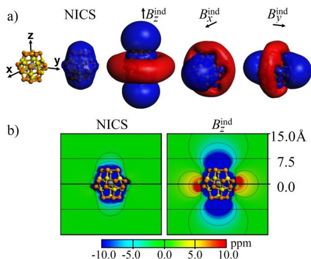
Fig. 3. Magnetic response properties of [\text{K}@\text{Au}_{12}\text{Sb}_{20}]^{5-} from NICS isosurfaces and under specific orientations of the external field accounting for \mathbf{B}^{\text{ind}}_z , \mathbf{B}^{\text{ind}}_{x,y} and \mathbf{B}^{\text{ind}}_y isosurfaces. Isosurfaces set at \pm 3.0 ppm, blue – shielding; red – deshielding.
