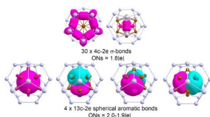
Fig. 5. Bonding pattern of [\text{Sn}@\text{Cu}_{12}@\text{Sn}_{20}]^{2-} . Copper atoms are brown. Reproduced with permission from reference 202 . Copyright Wiley, 2020.
