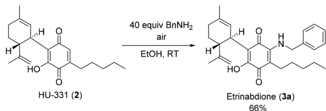
Scheme 2 Synthesis of Etrinabidione (3) via treatment of 2 with a large excess of benzylamine and subsequent aerobic oxidation with air.
