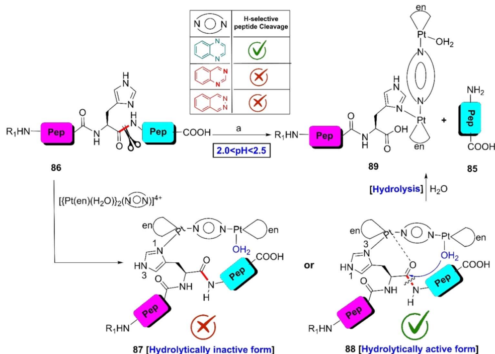
Scheme 14 H-selective cleavage of the peptide bond via metal complexation: role of ligands. Reaction conditions: (a) \text{D}_2\text{O} , \text{pH } 2.0 < \text{pH} < 2.5 , 37^\circ\text{C} .
