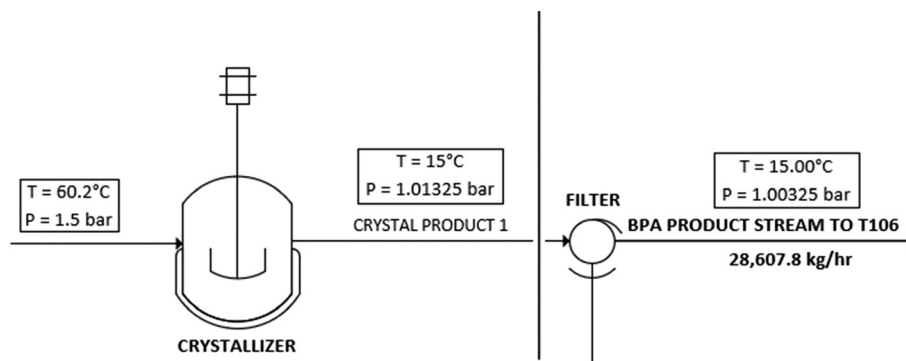
Fig. 4 PFD of the solid separation step of the process.
