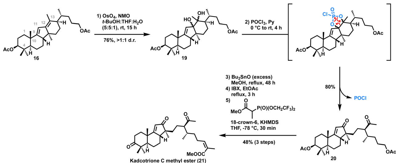
Scheme 3 Synthesis of kadcotrione C methyl ester.
