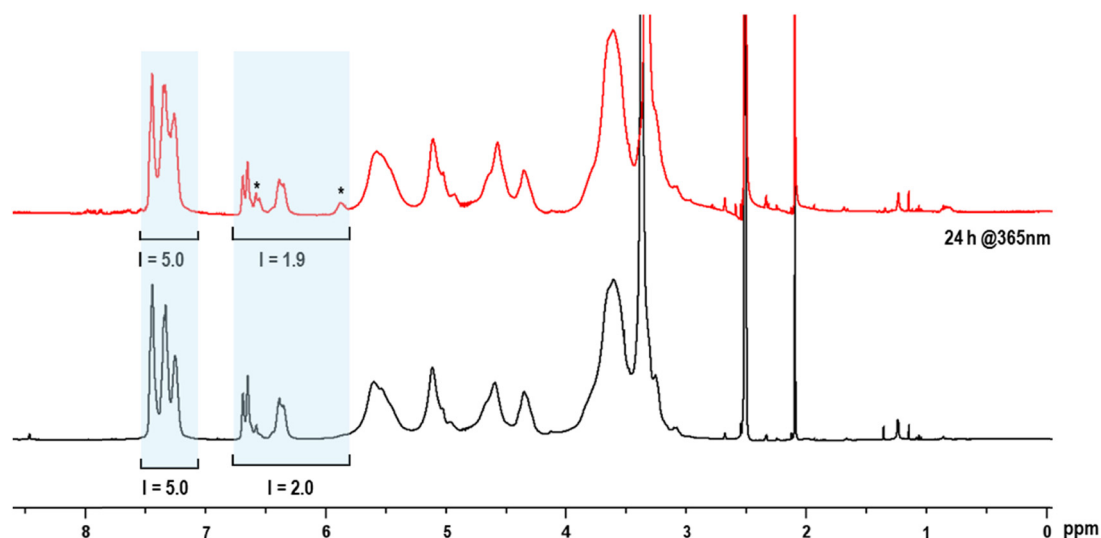
Fig. 7 ^1\text{H} -NMR spectra of the CS2 starch ether in DMSO- d_6 before and after 24 h UV exposure at \lambda \sim 365 nm. Shaded areas highlight changes in the spectra and * indicates new peaks; relevant integrals are indicated ( I ).
