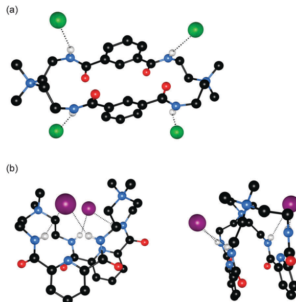
Fig. 2 (a) Crystal structure of 9 ^{2+} ·2Cl ^- ·2.66H _2 O (b) two views on the crystal structure of 10 ^{2+} ·2I ^- ·2H _2 O. Hydrogen bonds are shown as dashed lines; solvent molecules and non-coordinating hydrogens are omitted for clarity; chloride is represented in green spacefill; iodide in purple spacefill and the receptors are shown in ball-and-stick.
