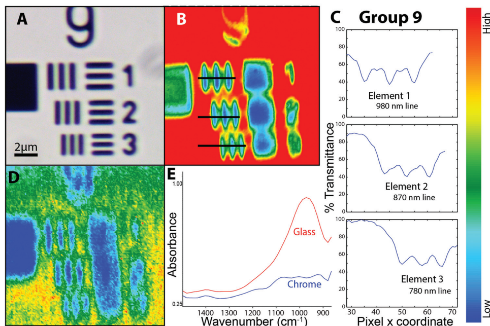
Fig. 2 FTIR-ATR images of elements in group 9 of the high spatial resolution 1951 USAF target. (a) Visible image of elements in group 9. (b) FTIR-ATR image (128 × 128 FPA) at high magnification (nominal 0.25 \times 0.25 \mu\text{m}^2 per pixel) processed as %T through glass at 3500 \text{ cm}^{-1} . (c) Line plot of %T at adjacent pixels extracted from image, across each element, shows that contrast exceeds sparrow criterion. Pixels extracted at locations shown in (b) as horizontal black lines. (d) FTIR-ATR image processed on integrated intensity of Si-O band. (e) Absorbance spectra taken from a single pixel on glass (red) and a single pixel on chrome bar (blue) showing Si-O band.
