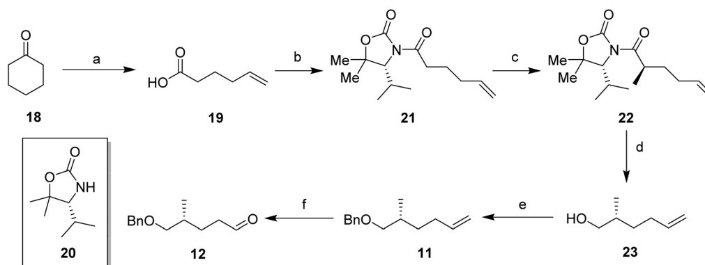
Scheme 2 Synthesis of chiral fragments 11 and 12 . Reagents and conditions: (a) (i) \text{H}_2\text{O}_2 , MeOH, 30 min. (ii) \text{FeSO}_4 \cdot 7\text{H}_2\text{O} , \text{CuSO}_4 \cdot 5\text{H}_2\text{O} , \text{H}_2\text{O} , 20%; (b) (i) Oxazolidinone 20 , n\text{BuLi} , THF, -78^\circ\text{C} , 30 min. (ii) Pivaloyl chloride, \text{NEt}_3 , THF, 0^\circ\text{C} , 30 min, r.t., 1.5 h, 93%; (c) NaHMDS, MeI, THF, -78^\circ\text{C} , 3 h, 92%, dr >98 : 2; (d) \text{LiAlH}_4 , \text{Et}_2\text{O} , 0^\circ\text{C} , 2 h, 66%; (e) NaH, BnBr, DME, r.t.-reflux, 20 h, 94%; (f) (i) \text{O}_3 , DCM, -78^\circ\text{C} . (ii) \text{PPh}_3 , -78^\circ\text{C} –r.t., 55%.
