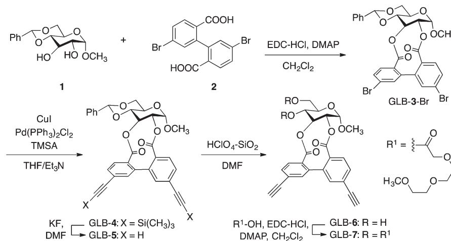
Scheme 1 Synthesis of GLB-7 bearing a glucose-linked biphenyl unit.
