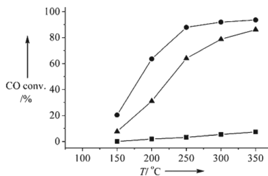
Fig. 9 WGS reaction “light-off” profiles for 1% Au on \text{CeO}_2 nanorods (●), cubes (■), and polyhedra (▲) (modified with permission from ref. 37, copyright 2008 Wiley-VCH).
