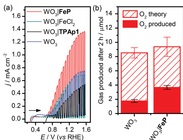
Fig. 3 (a) LSVs under chopped illumination (AM1.5G, 0.2 W \text{cm}^{-2} ) of \text{WO}_3 (blue line), \text{WO}_3 | FeP (red line), \text{WO}_3 | \text{FeCl}_2 (green line) and \text{WO}_3 | TPAp1 (black line) at \nu = 5 mV \text{s}^{-1} . (b) Amount of \text{O}_2 generated after two h PEC water oxidation by \text{nanoWO}_3 with and without FeP under solar illumination at E_{\text{appl}} = 1.0 V vs. RHE. The theoretical amount of \text{O}_2 was calculated based on 100% faradaic yield and the experimentally measured \text{O}_2 was quantified by a fluorescence probe. Conditions: a Ag/AgCl reference electrode and a Pt mesh counter electrode in aqueous \text{Na}_2\text{SO}_4 (0.1 M) solution at pH 3, \text{N}_2 atmosphere and room temperature.
