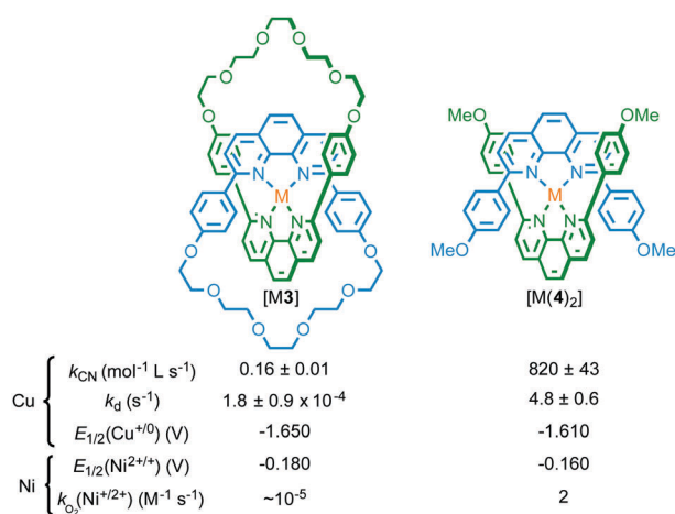
Fig. 2 Effect of the mechanical bond on the stability and electrochemistry of metal complexes of catenane [M(3)] compared with non-interlocked analogue [M(4)] . 5,8
