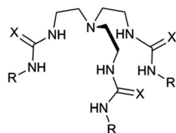
115 X=O R= \text{C}_6\text{H}_5 116 X=S R= \text{C}_6\text{H}_5 117 X=O R= \text{C}_6\text{F}_5 118 X=S R= \text{C}_6\text{F}_5 119 X=O R= m\text{-C}_6\text{H}_3(\text{CF}_3)_2 120 X=S R= m\text{-C}_6\text{H}_3(\text{CF}_3)_2
