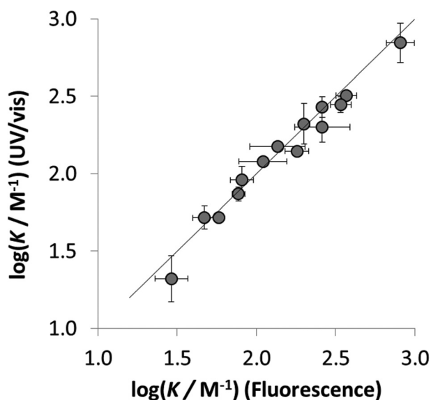
Fig. 3 Comparison of the \log(K/M^{-1}) measured for the H-bonded complexes 1-X using fluorescence emission spectroscopy and UV/vis absorption spectroscopy. The line represents \log(K/M^{-1}) (fluorescence) = \log(K/M^{-1}) (UV/vis).
