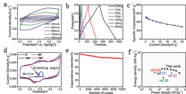
Fig. 5 (a) CV and (b) GCD curves of the symmetric SC in 1.0 M \text{H}_2\text{SO}_4 electrolyte in a two-electrode system. (c) Specific capacitances at various current densities. (d) CV curves of the GP@cc-based flexible SC at different bending angles. (e) Cycling behavior of the SC device at a current density of 5 \text{ A g}^{-1} . (f) Ragone plot of the SC device.
