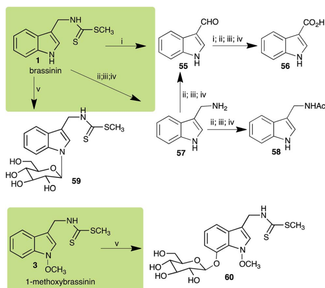
Scheme 1 Detoxification of the cruciferous phytoalexins brassinin (1) and 1-methoxybrassinin (3) by plant fungal pathogens: (i) Lep-tosphaeria maculans (canola virulent isolates), (ii) L. maculans (brown mustard virulent isolates) and L. biglobosa ; (iii) Alternaria brassicicola ; (iv) Botrytis cinerea ; (v) Sclerotinia sclerotiorum .
