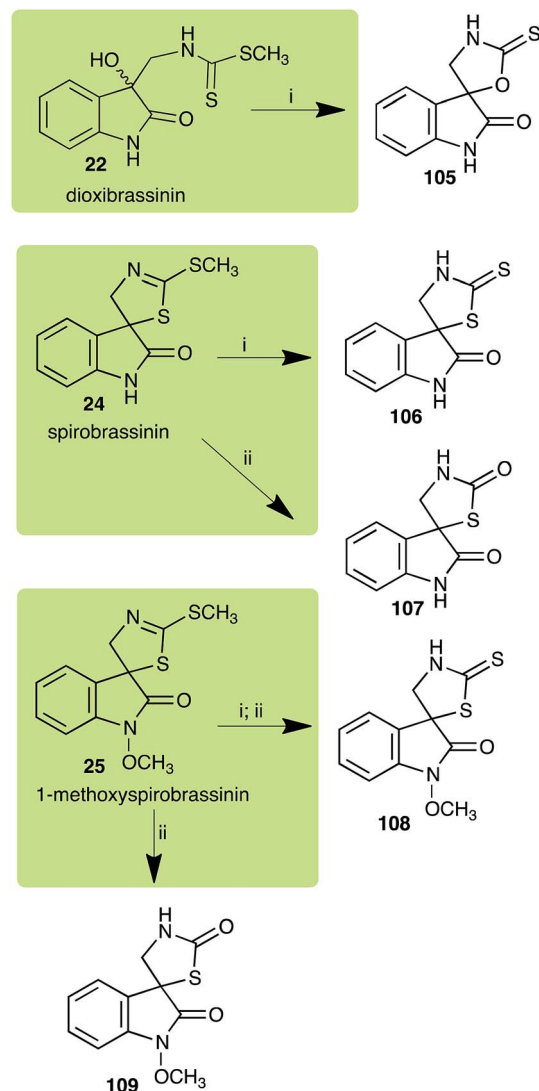
Scheme 7 Detoxification of the cruciferous phytoalexins dioxibrassinin ( 22 ), spirombrassinin ( 24 ) and 1-methoxyspirombrassinin ( 25 ) by plant fungal pathogens: (i) Leptosphaeria maculans (brown mustard virulent isolates); (ii) Sclerotinia sclerotiorum .
