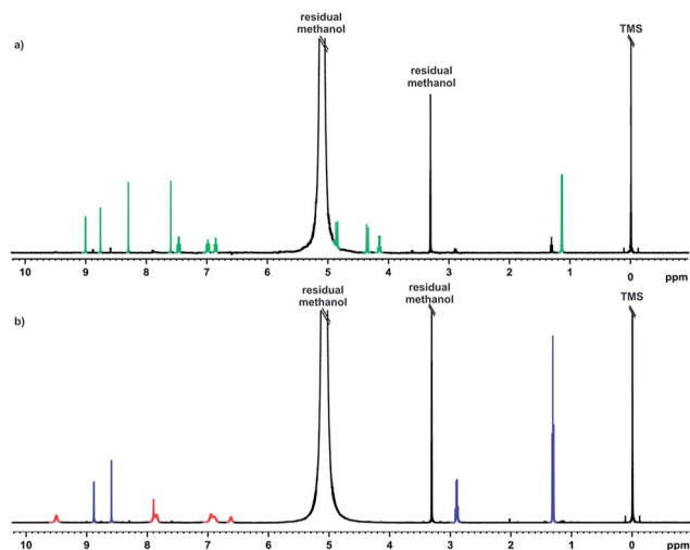
Figure 1 displays two ^1\text{H} NMR spectra. The top spectrum shows the chemical shifts (ppm) of degradation product 1 (red peaks) and degradation product 2 (blue peaks) in \text{CDCl}_3 . The bottom spectrum shows the same products with diffusion-ordered NMR (DOSY) data. The y-axis represents the diffusion coefficient ( 10^{-10} \text{ m}^2 \text{ s}^{-1} ) and the x-axis represents the chemical shift (ppm). Degradation product 1 is associated with a diffusion coefficient of approximately 2.1, and degradation product 2 is associated with a diffusion coefficient of approximately 5.2. Residual methanol and TMS are also labeled.
