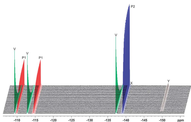
Figure 1 displays the diffusion NMR spectra of degradation products. The top panel shows the 1D ^1\text{H} NMR spectrum with peaks at 11.0 ppm (red), 11.2 ppm (red), and 13.9 ppm (blue). The bottom panel shows the 2D DOSY NMR spectrum with diffusion coefficients for degradation product 1 (red dotted line at \sim 2.2 \times 10^{-10} \text{ m}^2 \text{ s}^{-1} ) and degradation product 2 (blue dotted line at \sim 5.3 \times 10^{-10} \text{ m}^2 \text{ s}^{-1} ).
