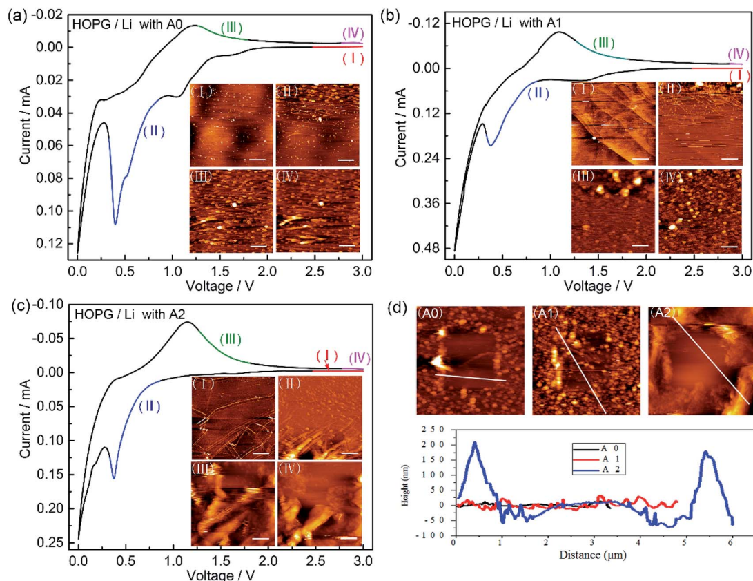
Fig. 3 In situ AFM images of HOPG electrode cycled at a scanning rate of 2 mV s -1 between 3.0 and 0.0 V with electrolytes A0 (a), A1 (b) and A2 (c). (I) 3.0–2.47 V; (II) 0.86–0.33 V; (III) 1.27–1.80 V; (IV) 2.87–3.0 V. The scanning directions are from bottom to top. The scales bars are 1 μm. (d) AFM images after scratching a 2.5 × 2.5 μm 2 area on the EEI covered surface from electrolytes A0, A1, and A2. The bottom shows line profiles indicated in (A0), (A1), and (A2).
