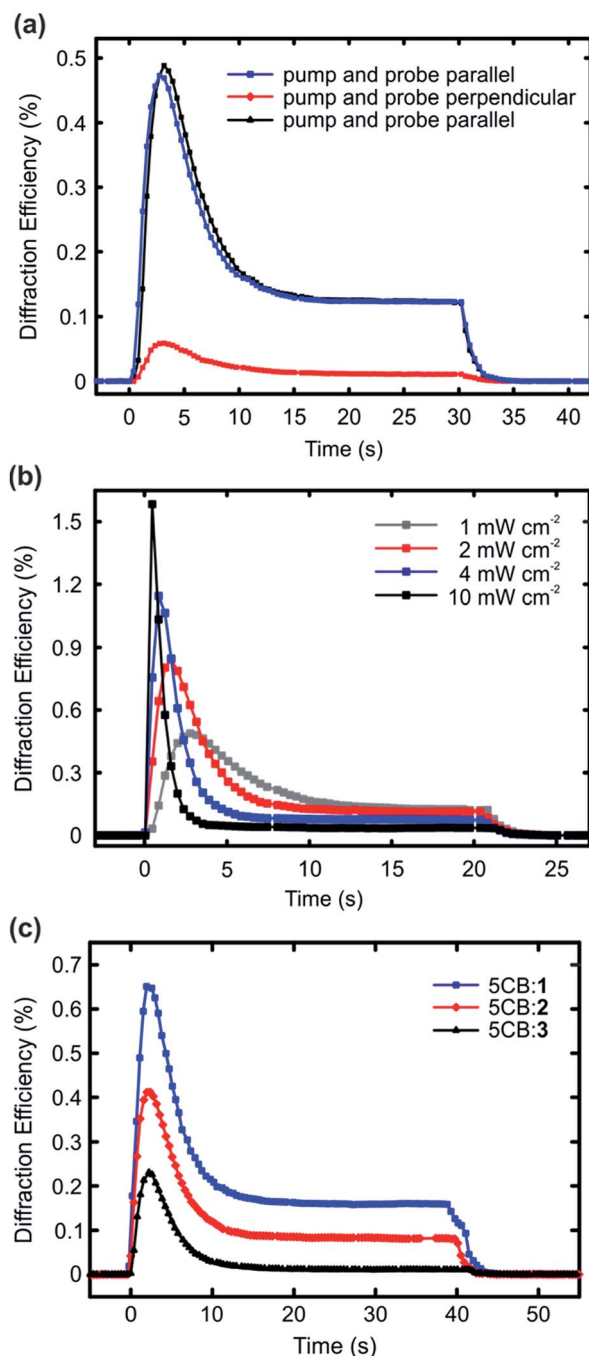
Fig. 3 (a) The effect of pump–probe polarization combination on the diffraction efficiency of 1 mol% 5CB:1 sample (488 nm; period: 40 \mu\text{m} ; intensity: 1 mW cm -2 for both interfering beams). (b) The intensity dependence of the diffracted signal for 1 mol% 5CB:1 sample (488 nm; period: 40 \mu\text{m} ; the intensities given represent the value for each interfering beam). (c) Diffraction efficiency curves for 10 \mu\text{m} planar cells of the 5CB:x mixtures upon exposure to interference pattern of two p -polarized 488 nm laser beams (period: 30 \mu\text{m} ; intensity: 1 mW cm -2 ). The irradiation is started at 0 s, and ceased at 30 s (a), 20 s (b), and 40 s (c), after which the diffracted signal quickly vanishes.
