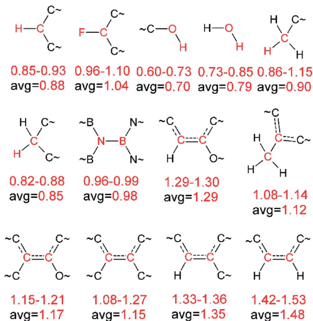
Fig. 9 The range and average of DDEC6 bond orders for thirteen different bond types. The directly connected (red) and adjacent connected (black) atoms defined each bond type. A tilde ( \sim ) indicates further bond connections to the remaining structure, but the specific form of these did not affect the bond type. Dashed lines indicate delocalized \pi -electrons. Each bond type displayed here occurred in at least five bonds distributed over at least two materials. DDEC6 bond orders for each bond type showed excellent transferability between different materials.
