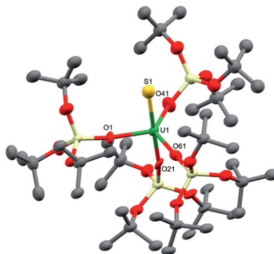
Fig. 5 Molecular structure of the anionic fragment of one of the crystallographically independent pairs of [\text{K}(\text{2.2.2-cryptand})][\text{US}\{\text{OSi}(\text{OTfBu})_3\}_4] in crystals of 8-15tol shown with 50% probability thermal ellipsoids. [\text{K}(\text{2.2.2-cryptand})]^+ , hydrogen atoms and lattice solvent molecules have been omitted for clarity.
