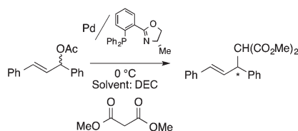
Scheme 28 Pd-Catalyzed asymmetric allylic alkylation in DEC.
