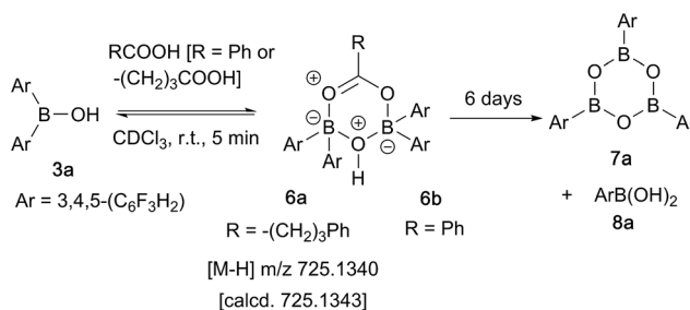
Scheme 5 Reaction of 3,4,5-trifluorophenylborinic acid 3a with benzoic acid or 4-phenylbutyric acid, resulting in boroxine formation.
