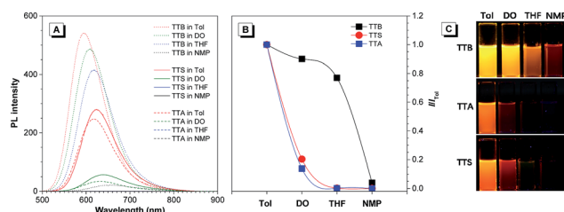
Fig. 1 (A) Emission spectra of TTB, TTS, and TTA in solvents with different polarities. Concentration: 10 \mu M; excitation wavelength: 480 nm. (B) Relative PL intensity ( I/I_{Tol} ) of TTB, TTA, and TTS in different solvents, where I_{Tol} = PL intensity in toluene and I = PL intensity in other solvents. (C) Fluorescence photographs of TTB, TTA, and TTS in different solvents taken under 365 nm UV illumination.
