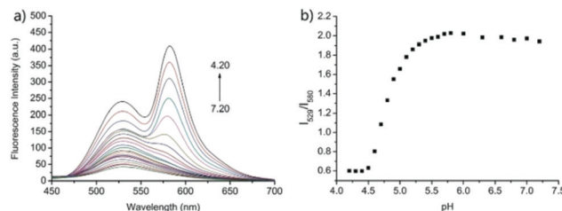
Fig. 23 (a) Fluorescence spectra of probe 18 (5 \mu M) in the B–R buffer/EtOH (9/1, v/v) solution at different pH values (7.20, 7.00, 6.80, 6.60, 6.30, 6.00, 5.80, 5.70, 5.60, 5.40, 5.30, 5.20, 5.10, 5.00, 4.90, 4.80, 4.70, 4.60, 4.50, 4.40, 4.30, and 4.20); and (b) the plot of the emission ratios of R at I_{529}/I_{580} versus pH values; \lambda_{\text{ex}} = 390 nm. Copyright 2015 Royal Society of Chemistry.
