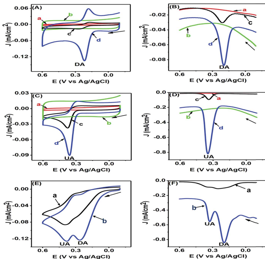
Fig. 7 CVs (A) and DPVs (B) of blank 0.1 M PBS solution of pH 7.0 (a and b) and 50 μM DA (c and d) in the same PBS of pH 7.0 at the GCE (a and c) and PTPCNs/GCE (b and d). CVs (C) and DPVs (D) of blank 0.1 M PBS of pH 7 (a and b) and 200 μM UA (c and d) in PBS of pH 7.0 at the GCE (a and c) and PTPCNs/GCE (b and d). CVs (E) and DPVs (F) of the mixture of 50 μM DA and 200 μM UA in 0.1 M PBS of pH 7.0 at the bare GCE (a) and PTPCNs/GCE (b).
