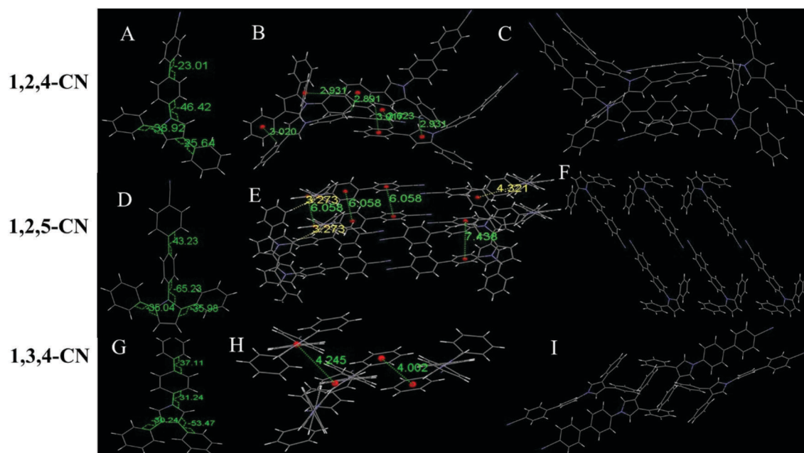
Fig. 4 (A) Molecular structure, (B) interaction distances of C–H... \pi interactions and (C) stacking image of 1,2,4-CN. (D) Molecular structure, (E) interaction distances of C–H... \pi interactions and (F) stacking image of 1,2,5-CN. (G) Molecular structure, (H) interaction distances of face-to-face phenyl rings and (I) stacking image of 1,3,4-CN. Gray color corresponds to carbon, white to hydrogen and blue to nitrogen.
