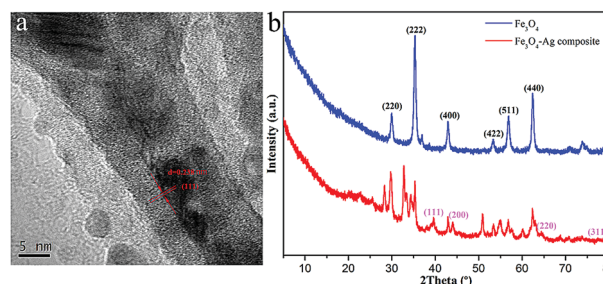
Fig. 4 HRTEM image of Ag nanowires (a) and XRD patterns of the \text{Fe}_3\text{O}_4\text{-Ag} nanocomposite (b).
