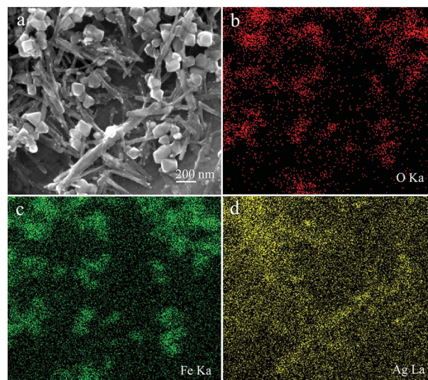
Fig. 3 SEM image (a) and O/Fe/Ag (b, c, and d) elemental mapping of the obtained \text{Fe}_3\text{O}_4\text{-Ag} nanocomposite.
