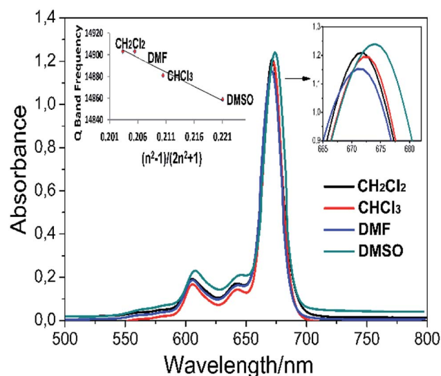
Fig. 5 Absorption spectra of complex 5 in various solvents ( \sim 15 \times 10^{-6} mol \text{dm}^{-3} ). The inset exhibits a plot of the Q band frequency of complex 5 against the function (n^2 - 1)/(2n^2 + 1) , where n is the solvents' refractive index.
