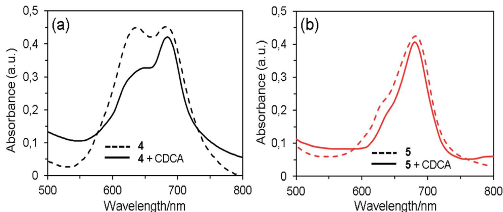
Fig. 3 UV-Vis absorption spectra of 4 (a) and 5 (b) without and with 1 mM CDCA on \text{TiO}_2 film.
