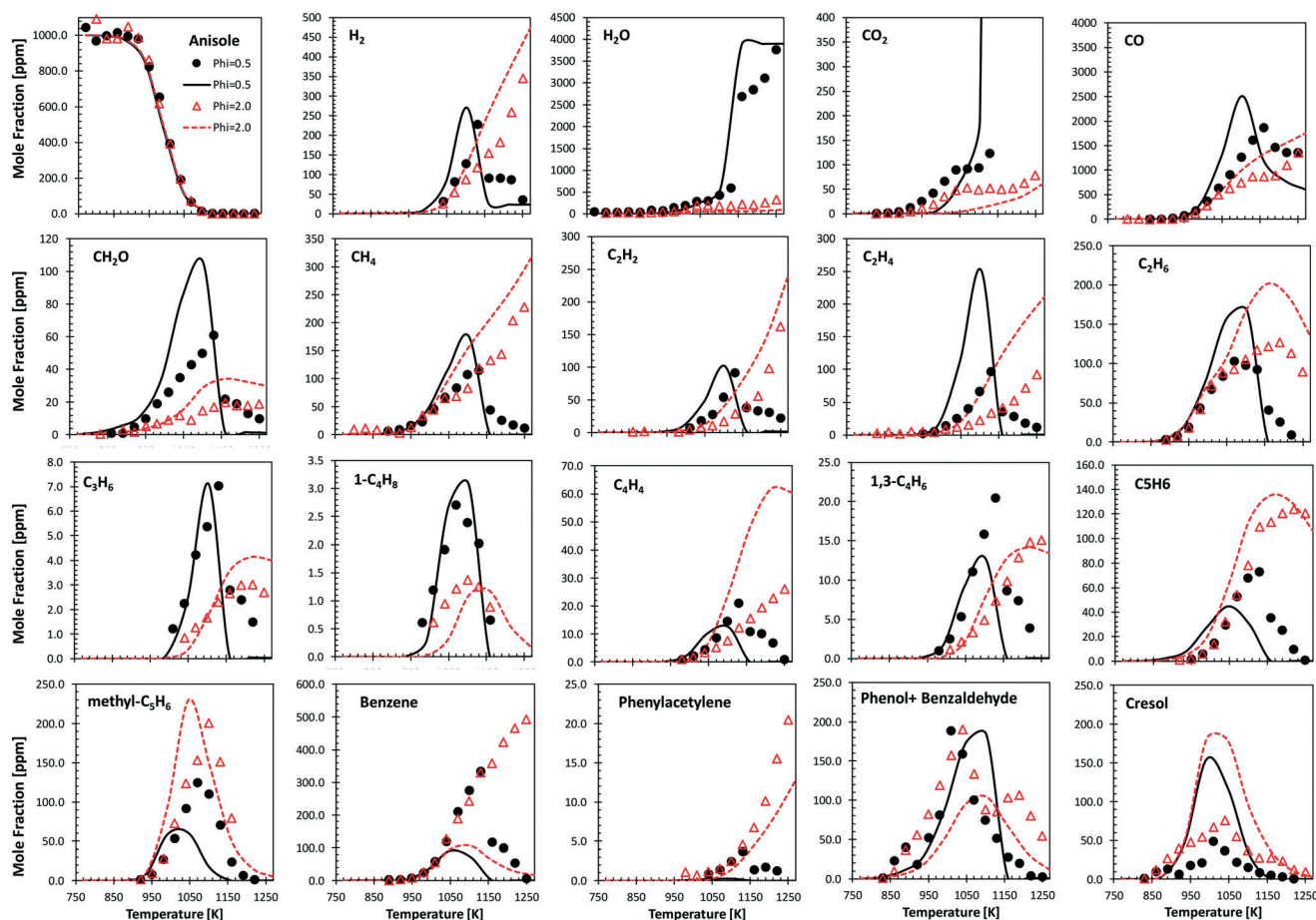
Fig. 9 Anisole atmospheric pressure oxidation in an Orleans JSR. 75 0.1% anisole/ \text{O}_2/\text{N}_2 mixtures under rich ( \phi = 2.0 , triangles) and lean conditions ( \phi = 0.5 , circles). Comparisons between experimental data (symbols) and model predictions (lines).
