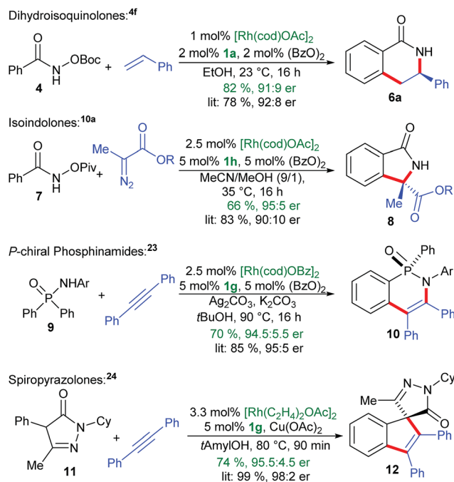
Scheme 6 Application of in situ \text{Cp}^x\text{Rh} -catalyst assembly under different benchmark reactions. Ar = 3,5- \text{CF}_3 - \text{C}_6\text{H}_3 , R = \text{CH}(\text{iPr})_2 .
