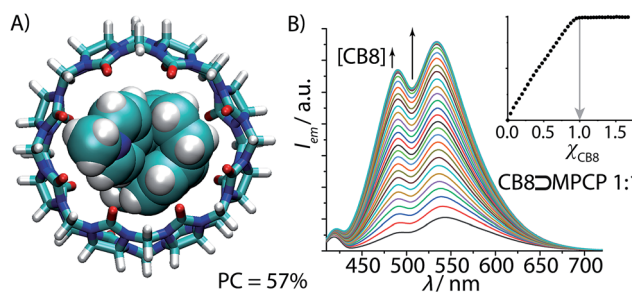
Fig. 4 (A) Geometry-optimized DFT model of the ground-state of CB8 \supset MPCP featuring an ideal packing coefficient (PC) of 57%. (B) Fluorescence spectra of MPCP ( \lambda_{\text{exc}} = 335 \text{ nm} , \lambda_{\text{em}} = 535 \text{ nm} , c = 1.9 \mu\text{M} ) in water with increasing CB8 concentration (0–3.1 \mu\text{M} ). The obtained binding isotherm (inset) allows us to deduce the stoichiometry (1 : 1) and the assessment of a very strong binding ( \log K_a \geq 9 ) (for accurate determination of K_a see Fig. 5 and Table 1).
