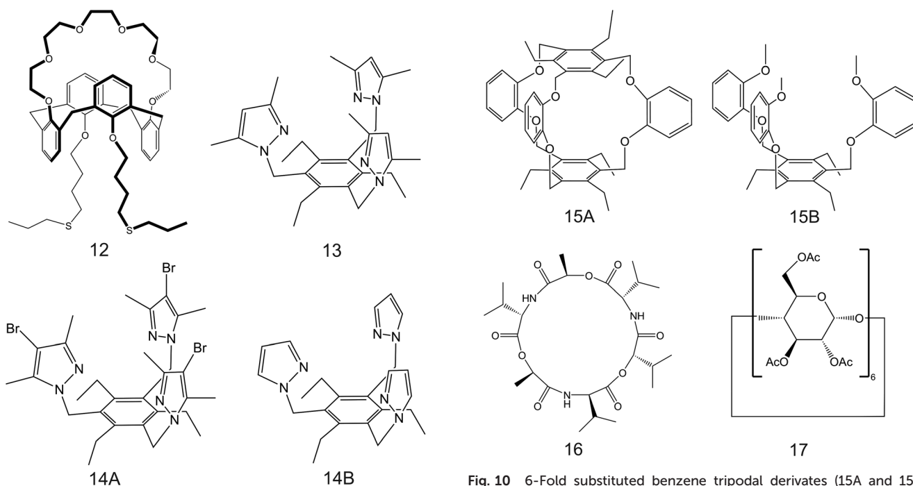
Fig. 9 Calix[4]arene-crown-6 (12) functionalized with alkyl sulfide units reported in the work of Saipina and co-workers. 93 The 6-fold substituted benzene tripod derivatives, reported in the works of Chin et al. (13; 80 14A and 14B 95 ), as \text{NH}_4^+ ionophores.
