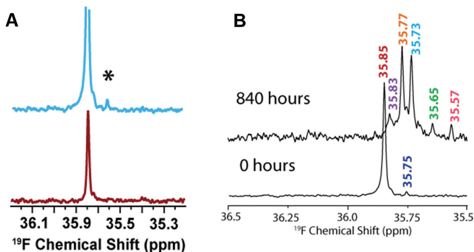
Fig. 6 (A) Characterization of A \beta_{1-40} oligomers using ^{19}\text{F} NMR. Fluorinated A \beta_{1-40} -tfM _{35} showing the presence of an additional peak (denoted as *) for a freshly prepared 182 \mu\text{M} peptide sample (blue) as compared to 46 \mu\text{M} sample (red). The small additional peak indicates A \beta_{1-40} -tfM _{35} oligomerization. The intensities of both samples are normalized to an internal TFE standard. (B) Monitoring the aggregation behavior of 182 \mu\text{M} A \beta_{1-40} -tfM _{35} by ^{19}\text{F} NMR at two different time intervals. The appearance of multiple peaks at 840 hours indicates the presence of variable sized A \beta_{1-40} -tfM _{35} species. Copyright © 2013, American Chemical Society. This figure is reproduced with permission from DOI: 10.1021/bi400027y; Biochemistry 2013, 52 , 1903–1912. Further details can be found in the published study. 115
