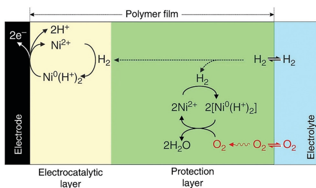
Fig. 13 A chemically inert polymer (PGMA-BA-PEGMA) is used to immobilize Dubois' Ni bis-diphosphine with glycine complex [\text{Ni}(\text{P}^{\text{Cy}}\text{N}_2^{\text{Gly}})_2]^{2+} on the surface of the electrode and prevent electrical contact between the metal complexes located within the polymer and the electrode. Two distinct regions are created: in the inner region (electrocatalytic layer), the Ni complex oxidizes \text{H}_2 , while in the outer region (protection layer), \text{Ni}^0 reduces \text{O}_2 to \text{H}_2\text{O} using the electrons produced from \text{H}_2 oxidation in the inner region. Reprinted with permission from ref. 280. (Creative Commons Attribution 4 International License).
