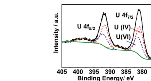
Fig. 6 High resolution U 4f XPS spectrum of uranium dioxide nanoparticles derived from the microwave decomposition of the uranyl EG gel. The spectrum was fitted with peaks of U(IV) and U(VI) (dashed lines).
