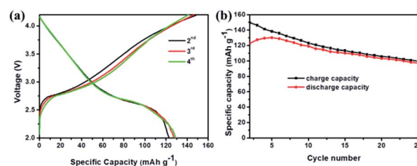
Fig. 8 Electrochemical performance of the assembled Sb@Sb 2 O 3 /3DNC||NCM622 full cell: (a) the second to fourth cycle charge/discharge curves at 100 mA g -1 , (b) cycling performance at a current density of 100 mA g -1 .
