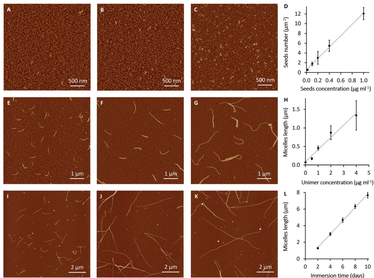
Fig. 2 AFM images of seeds and fibre-like micelles of PFDMS 44 - b -PDMS 250 - b -P3OT 17 on gold surfaces. The gold coated silicon slides were immersed for 2 h in seeds solution (A) 0.02\ \mu\text{g ml}^{-1} , (B) 0.1\ \mu\text{g ml}^{-1} and (C) 1\ \mu\text{g ml}^{-1} . (D) Variation in number of seeds as function of seeds solution concentration. (E–G) The micelles were grown from 0.02\ \mu\text{g ml}^{-1} immobilised seeds on Au surfaces by immersion for 1 day in unimer solutions with concentrations (E) 1, (F) 2 and (G) 4\ \mu\text{g ml}^{-1} . (H) Variation in length of micelles after 1 day as a function of unimer solution concentration. (I–K) Slow growth of the micelles from 0.005\ \mu\text{g ml}^{-1} seeds on gold surfaces and immersion in 0.5\ \mu\text{g ml}^{-1} of unimers solution for (I) 2, (J) 6 and (K) 10 days. (L) Variation in length of micelles as function of immersion time.
