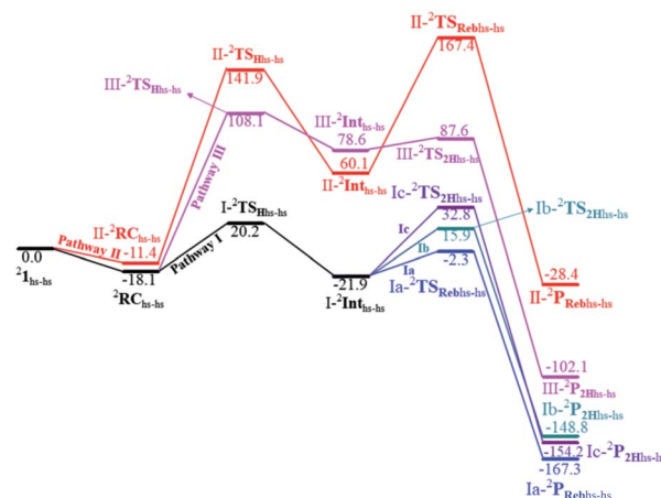
Fig. 6 Potential energy surface computed (energies are in \text{kJ mol}^{-1} ) for C–H activation of cyclopentane by species 2^1_{\text{hs-hs}} comparing the lowest estimate of barrier heights obtained from various pathways computed in Scheme 2.
