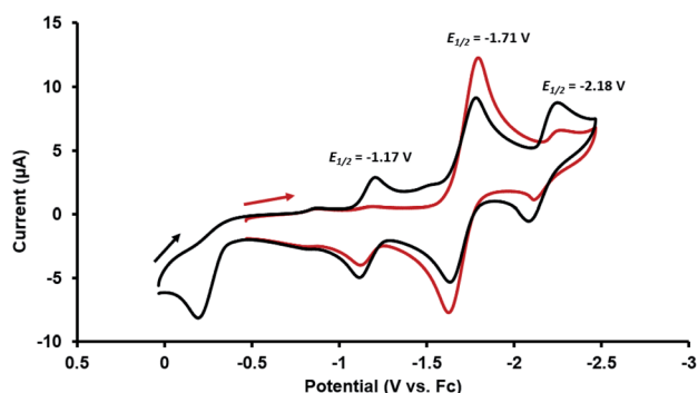
Fig. 2 Cyclic voltammograms of 2 (in 0.3 M [ ^t Bu 4 N][PF 6 ] in THF; scan rate: 100 mV s -1 ) scanning cathodically starting from the open circuit potential (red) and starting from 0 V (black) vs. Fc/Fc + .
