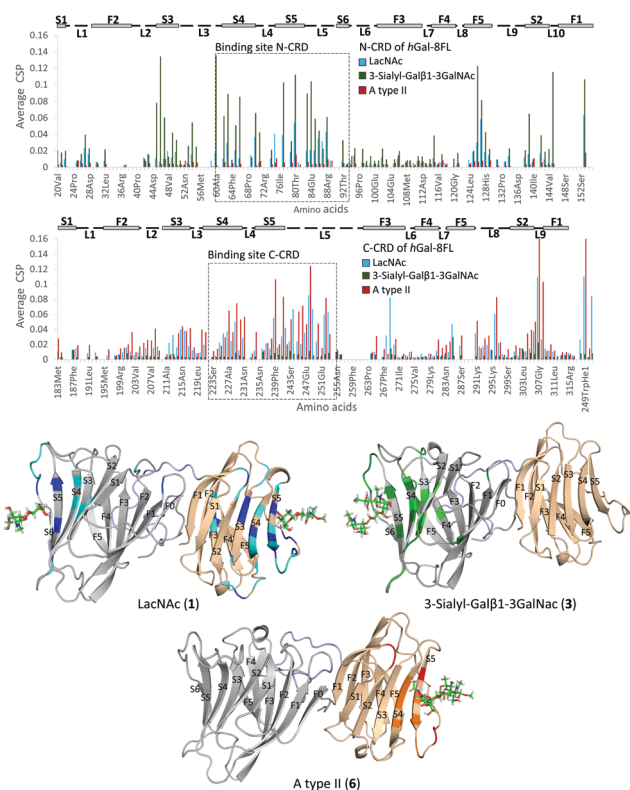
Fig. 5 Top, CSP analysis for 1 (blue, 60 equivalents), 3 (green, 10 equivalents) and 6 (red, 8 equivalents). Below, 3D models for the interaction of Gal-8FL with 1, top-left; 3, top-right; 6, below. The most perturbed residues are highlighted in dark (perturbed >2\sigma ) and light (perturbed >\sigma ) colors.
