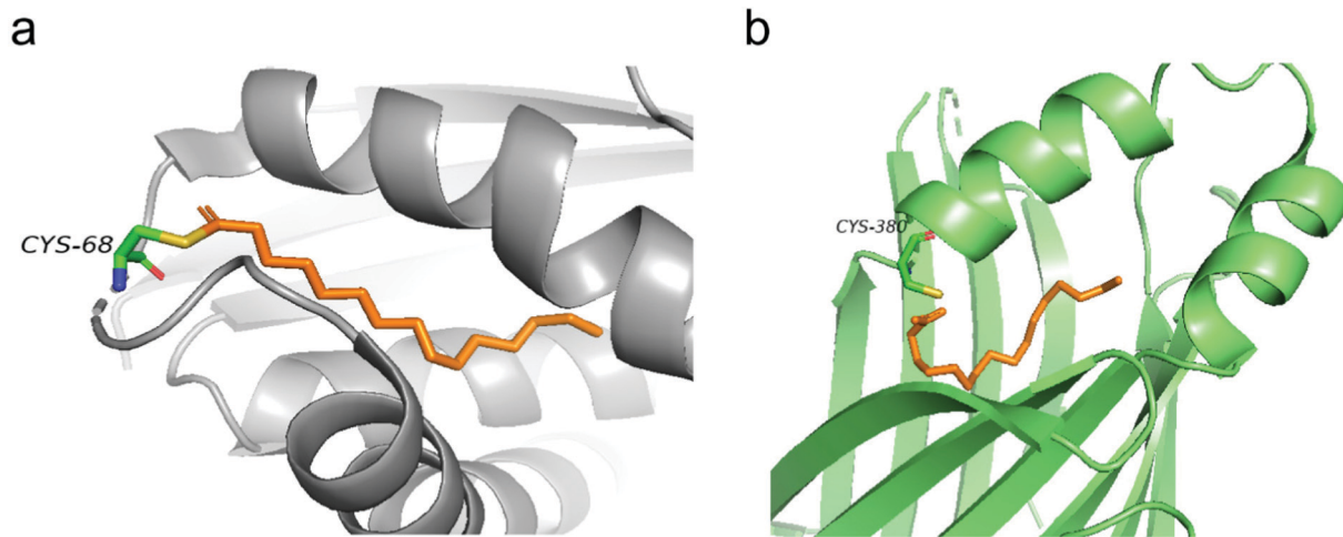
Fig. 2 (a) Palmitate (orange) covalently attaches to C68 in the structure of human Bet3 (PDB code 1SZ7). (b) Crystal structure of human TEAD2 YBD bound with palmitate (orange) (PDB code 5HGJ).
