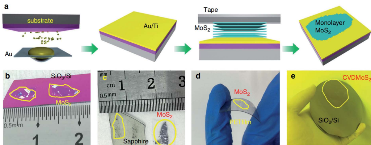
Fig. 1 Mechanical exfoliation of different monolayer materials with macroscopic size. (a) Schematic of the exfoliation process. (b–d) Optical images of exfoliated \text{MoS}_2 on \text{SiO}_2/\text{Si} , sapphire, and plastic film. (e) 2-inch CVD-grown monolayer \text{MoS}_2 film transferred onto a 4-inch \text{SiO}_2/\text{Si} substrate. 30 Reproduced with permission from ref. 30, copyright 2020 Springer Nature.
