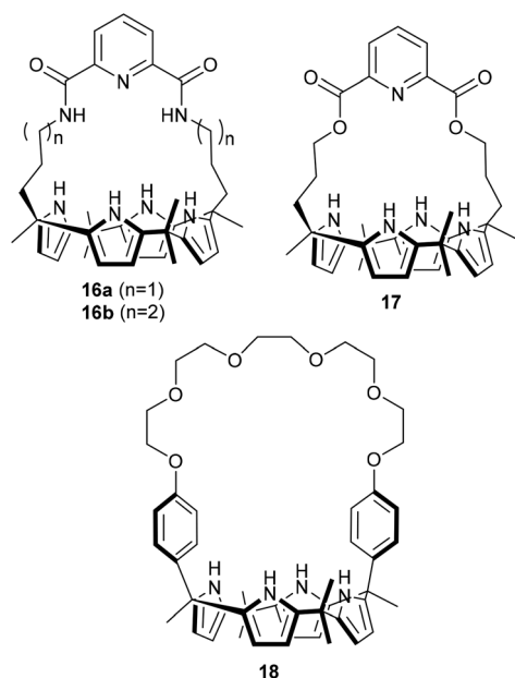
Fig. 10 Amides ( 16a,b ) and ester ( 17 ) strapped calyx[4]yrroles studied by Gale, Sessler and Shin 75 and calix[4]pyrrol-oligoether conjugate 18 described by Lee, Sessler and Gale. 76
