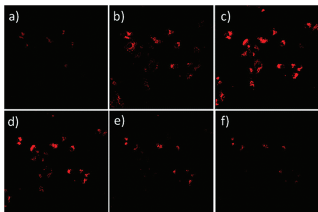
Fig. 3 Time-dependent fluorescence of U87MG cells stimulated by nigericin and observed under confocal fluorescence microscope using TAC-TFC: (a) t = 0 (before the addition of nigericin) (b–f) t = 1, 3, 5, 10 and 15 min, respectively, after the addition of nigericin. Adapted with permission from ref. 39, copyright American Chemical Society.
