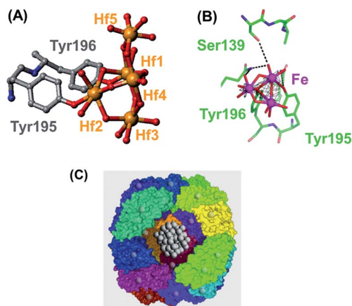
Fig. 16 (A) A pentanuclear oxo-Hf(IV) cluster in the open interdomain cleft of bacterial transferrin (Fbp), bound to the protein by two tyrosinate side-chains, Tyr195 and Tyr196 (adapted from Alexeev et al. , 2003). 104 This cluster can also be capped by phosphate. (B) Trinuclear \text{Fe}_3\text{O}_4 oxo-iron cluster in \text{Fe}_3\text{-Fbp} . The phenolate oxygen of Tyr196 is a central \mu^3 -bridging oxygen and Tyr195 is monodentate (adapted from Zhu et al. , 2003). 105 (C) The ferrihydrite-like ( \text{Fe}(\text{O})\text{OH} ) mineral core in the \text{Fe}(\text{III}) storage protein ferritin. Part of the 24 subunit protein shell has been cut away to show the ferrihydrite inside. Courtesy of Allen D. Elster, https://MRIquestions.com .
