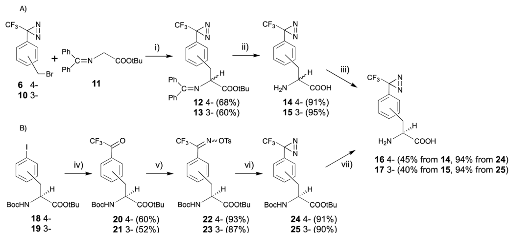
Fig. 4 Synthesis of (3- and 4-trifluoromethyldiaziriny)-D-phenylalanine derivatives. (i) \text{CsOH} , \text{Bu}_4\text{NBr} , \text{CH}_2\text{Cl}_2 , rt, 12 h, (ii) \text{TFA} , rt, 2 h, (iii) \text{L-amino acid oxidase} , pH 7.0, 37^\circ\text{C} , 12 h, (iv) (1) \text{MeLi} , (2) \text{tBuLi} , (3) \text{CF}_3\text{CO}_2\text{Et} , toluene, -78^\circ\text{C} , 12 h, (v) (1) \text{NH}_2\text{OH}\cdot\text{HCl} , pyridine, 70^\circ\text{C} , 1.5 h, (2) \text{TsCl} , TEA, acetone, rt, 1 h, (vi) \text{NH}_3 (l), ether, 80^\circ\text{C} , 9 h, (vii) \text{TFA} , rt, 8 h.
