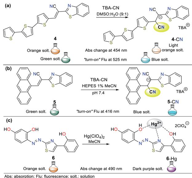
Fig. 2 Probes based on thiazoles for \text{CN}^- sensing in (a) \text{DMSO} : \text{H}_2\text{O} and (b) in HEPS solution (1% MeCN as a co-solvent), and (c) for \text{Hg}^{2+} recognition.
