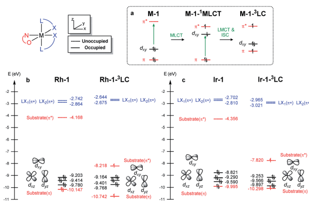
Fig. 7 (a) Electronic excitations and (b) frontier molecular orbitals of M-1 computed at the B3LYP-D3/cc-pVTZ(-f)/LACV3P** level of theory.
